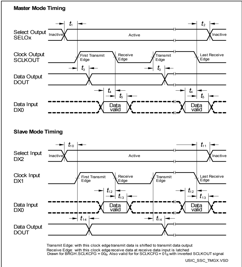
Figure 18 USIC - SSC Master/Slave Mode Timing
