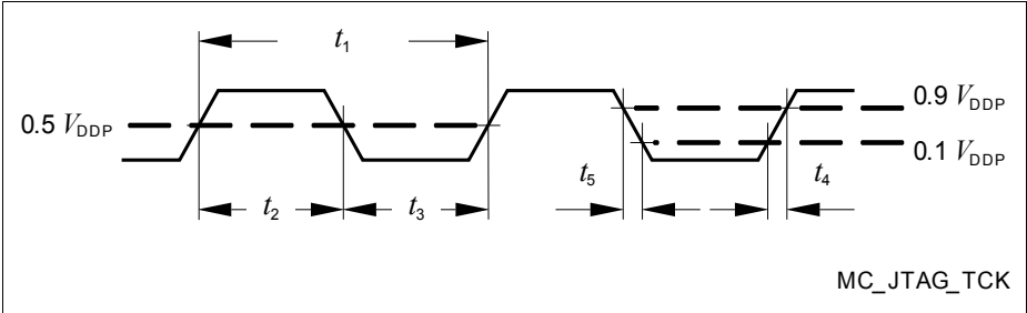
Figure 22 Test Clock Timing (TCK)
