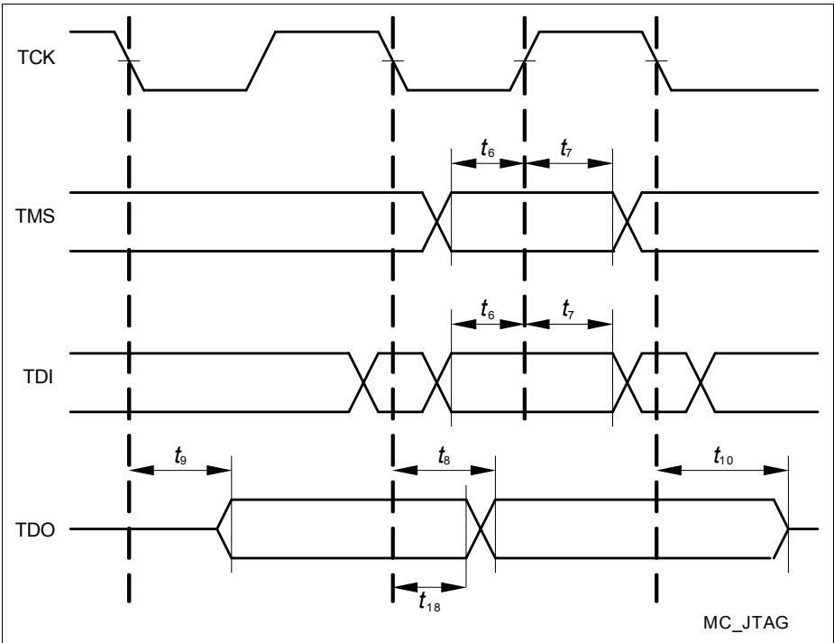
Figure 23 JTAG Timing
