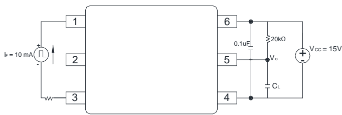
Figure 5 : Propagation Delay Test Circuit.
