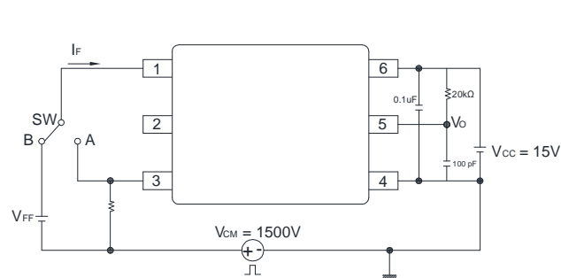
Figure 6 : CMR Test Circuit and Waveforms
