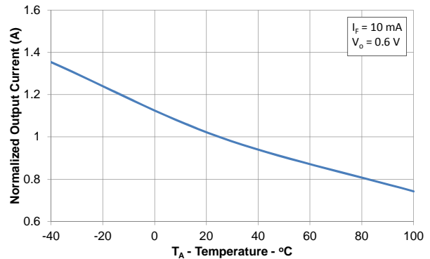
Figure 2: Normalized Output Current vs. Temperature
